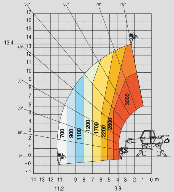
ROTATION ON STABILISERS WITH 3T WINCH
