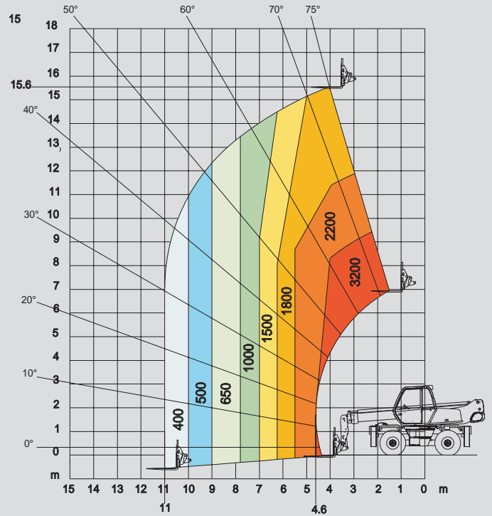
ROTATION ON STABILISERS WITH 3T WINCH
