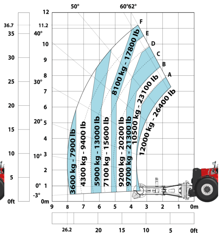
Machine on tyres with tyre handler TH 63 (Imperial)
