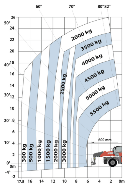
Machine on tires with forks Metric
