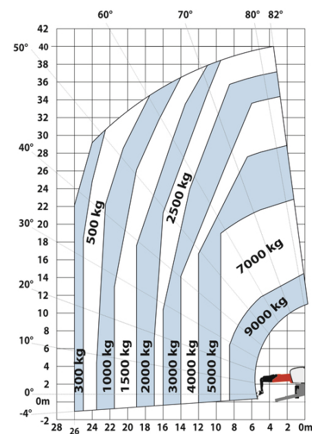
Machine on lowered stabilisers with hook 9000 kg (Metric)
