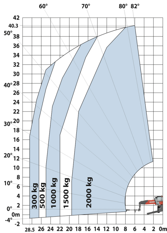
Machine on lowered stabilisers with 2000 kg jib (Metric)
